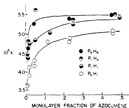
Figure 4. Effect of monolayer fraction and type of silica on the first-order decomposition rate constants. The independent variables are P_0 and P_1 , low and high purity silica, H_0 and H_1 , low and high density of surface OH groups.
